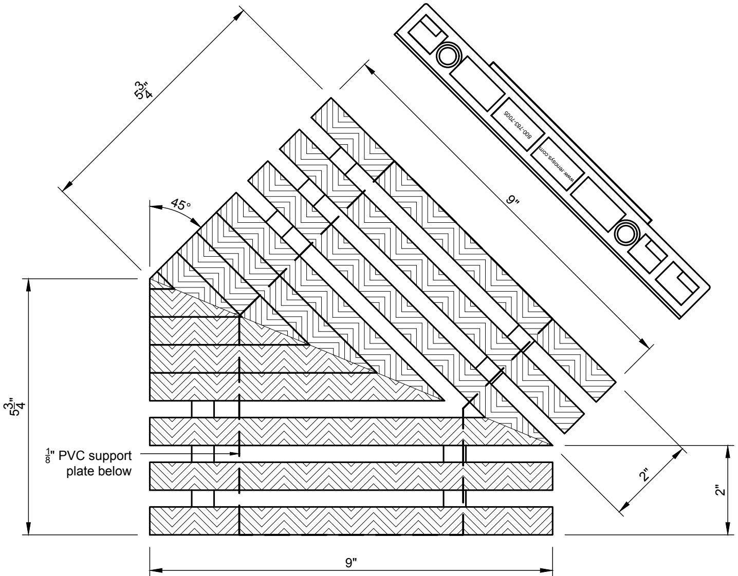
Top View
