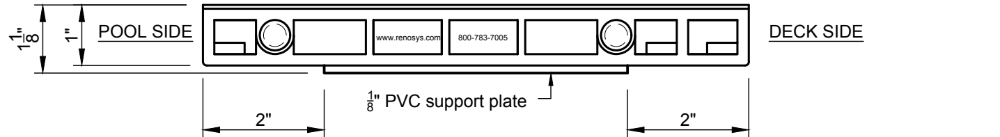
Side View
