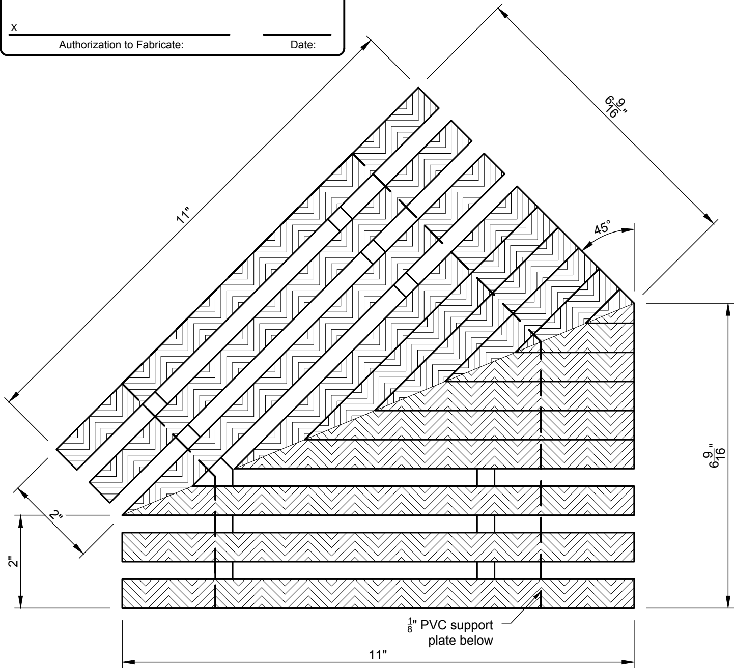
Top View
