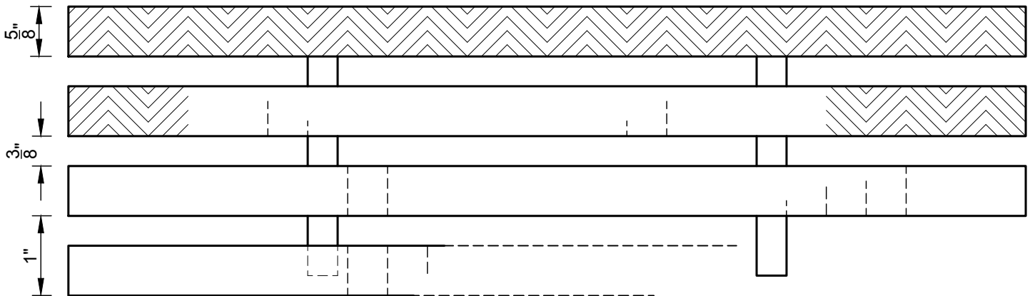
Top View
